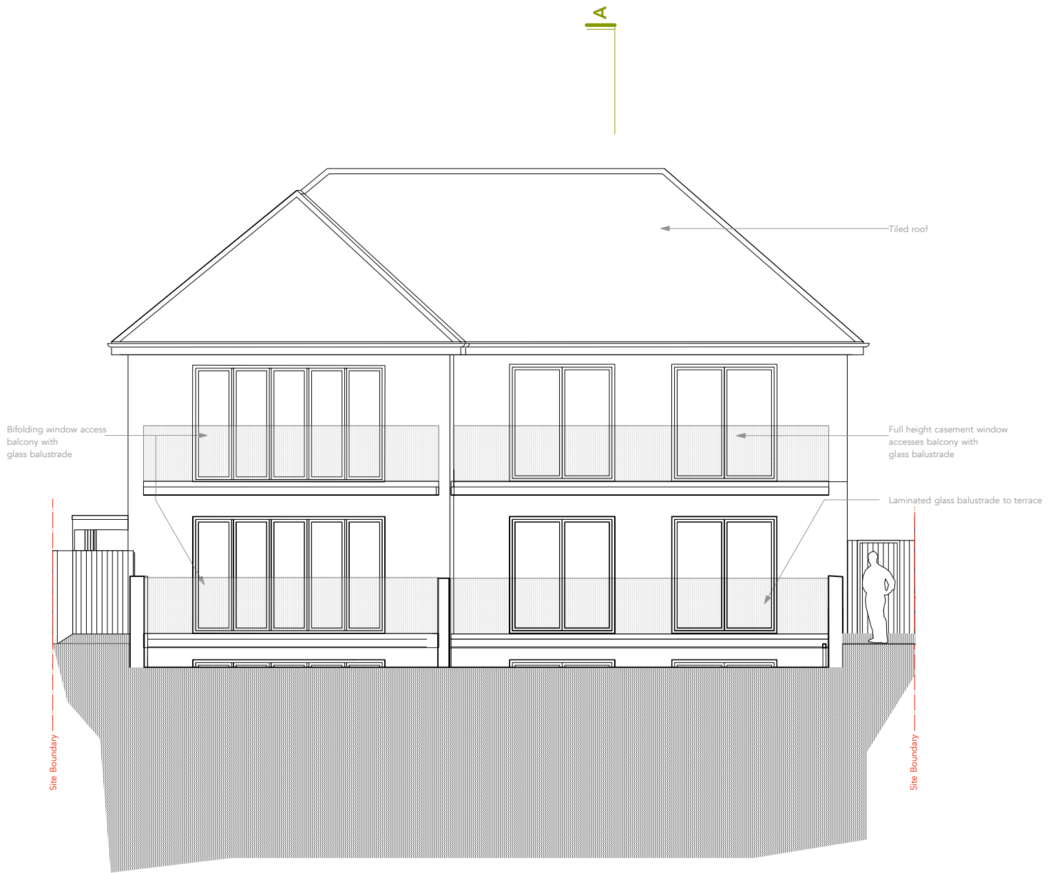
ELE Proposed Rear Elevation (Garden View)
